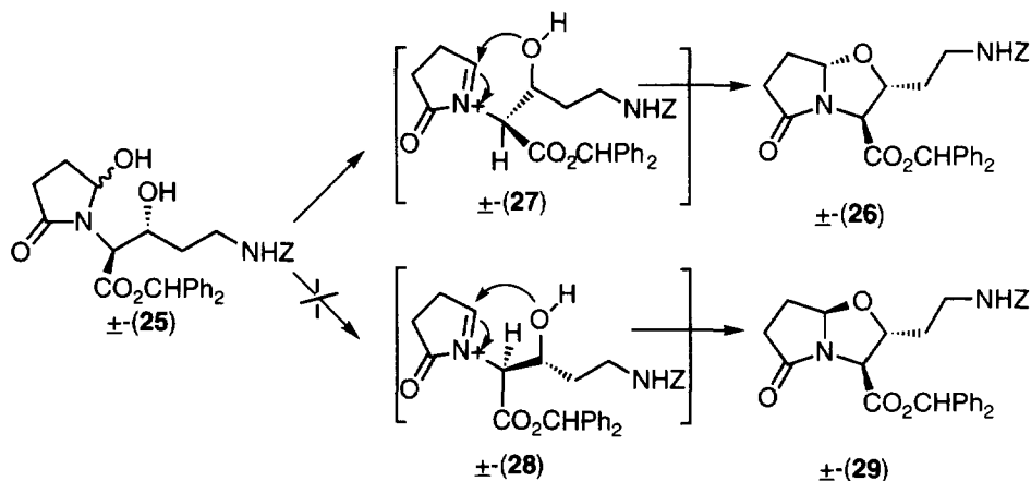
Scheme 6: Possible explanation for observed diastereoselectivity during the ring-closure reaction of ( 25 )
