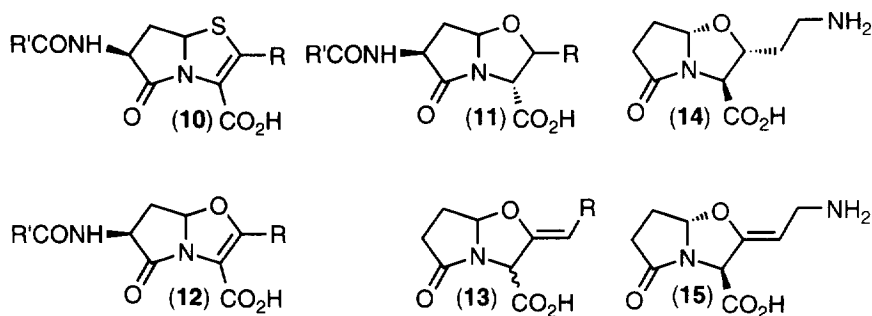
Scheme 2: Synthesis of \gamma -lactams
