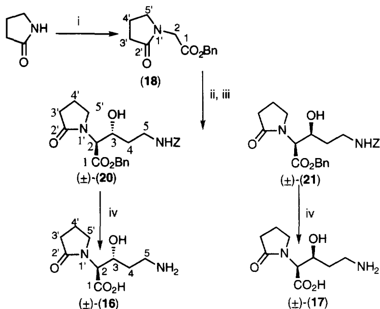
Scheme 3: Synthesis of \gamma -lactam substrates (16) and (17). Z = PhCH 2 OCO, Bn = PhCH 2 . Reagents: i). NaH, DMF, BrCH 2 CO 2 Bn; ii). (Me 3 Si) 2 NLi, THF, -78°C; iii). OHC(CH 2 ) 2 NHZ (19), then H 3 O + ; iv). H 2 , 10% Pd/C, EtOH-H 2 O (7:3)
