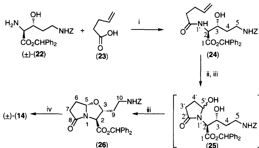
Scheme 5: Synthesis of the saturated \gamma -lactam intermediate ( 14 ). Z = PhCH 2 OCO; Reagents: i). 2-ethoxy-1-ethoxycarbonyl-1,2-dihydroquinoline, CH 2 Cl 2 ; ii). NaIO 4 , OsO 4 (cat.), THF, H 2 O (3:1); iii). CH 2 Cl 2 , CF 3 CO 2 H (cat.); iv). H 2 , Pd/C, EtOH / H 2 O (3:7)
