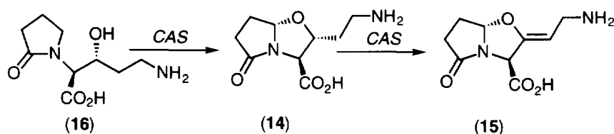
Scheme 4: The conversion of (16) to (14) and (15)
