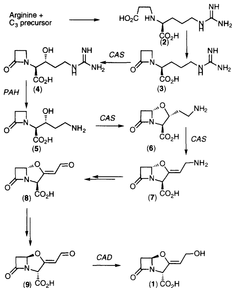
Scheme 1: biosynthesis of clavulanic acid (1), PAH = proclavaminic acid amidinohydrolase;
